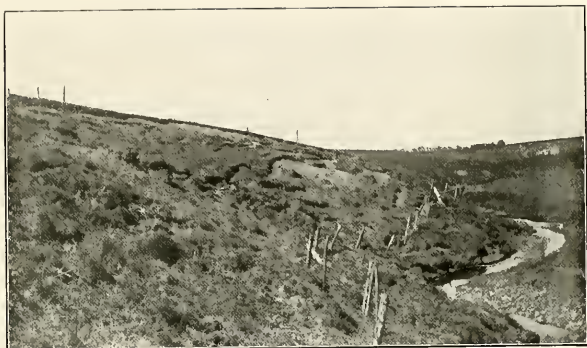
A. The widening of a valley by slumping.
